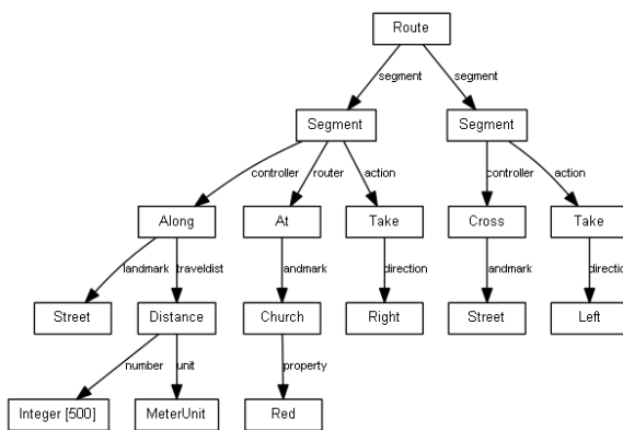
Figure 3: A conceptual route graph representing “follow the street for five hundred meters up to eh the red church then go right cross the street and turn left”
